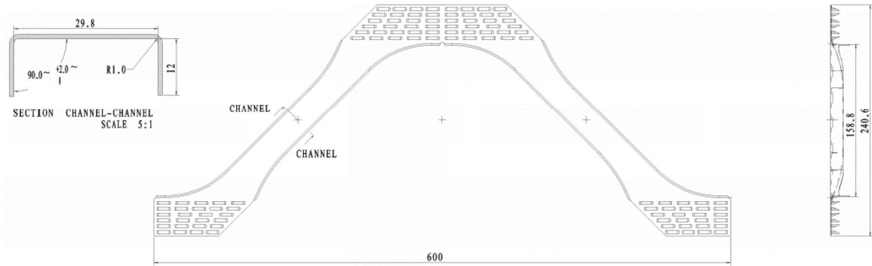
Figure A 6-4: PS10+
