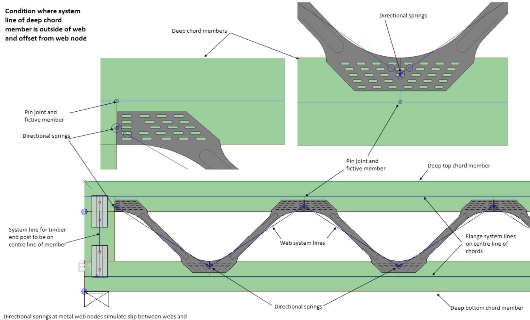
Figure A 2-3: Structural Model for Metal Web Beams and Columns with Single Webs - (Not to Scale)
