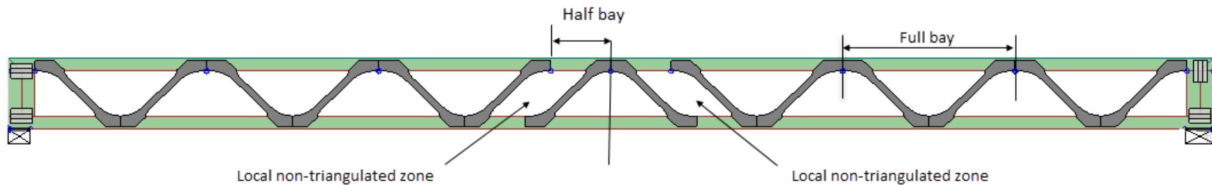
Figure A 1-8: Joist length achieved by locally discontinuing the metal-web triangulation
