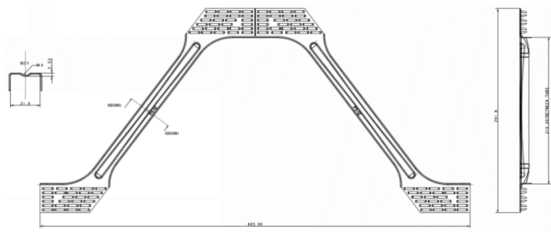
Figure A 6-5: PS12
