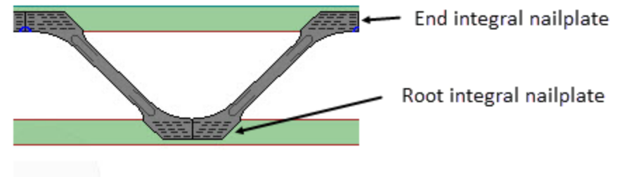
Figure A 1-3: Elevation on a single metal V-web
